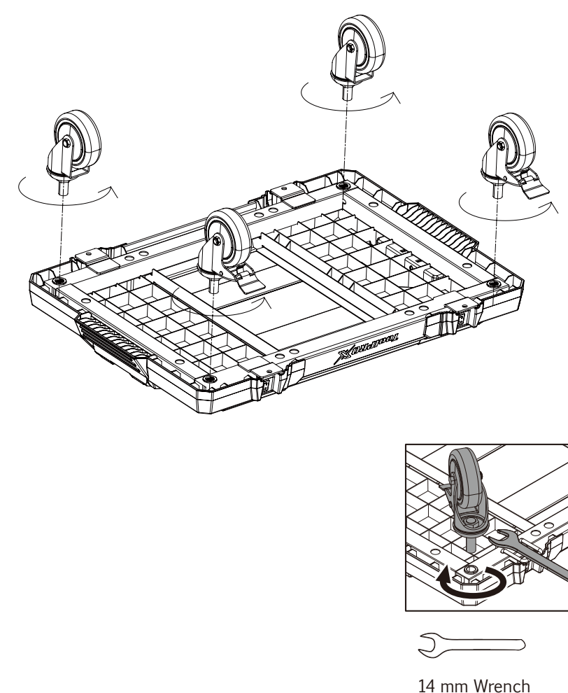
14 mm Wrench
