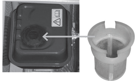
Fuel tank filter under fuel tank cap
